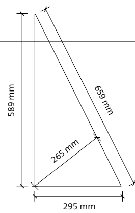
Triangle C1 659 x 265 mm
