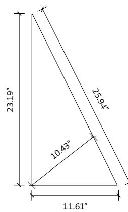
Triangle C1 25.94 x 10.43 inch
