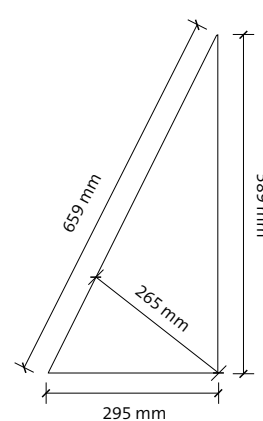
Triangle C2 265 x 659 mm
