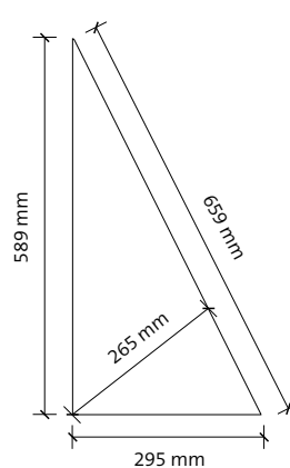
Triangle C1 659 x 265 mm
